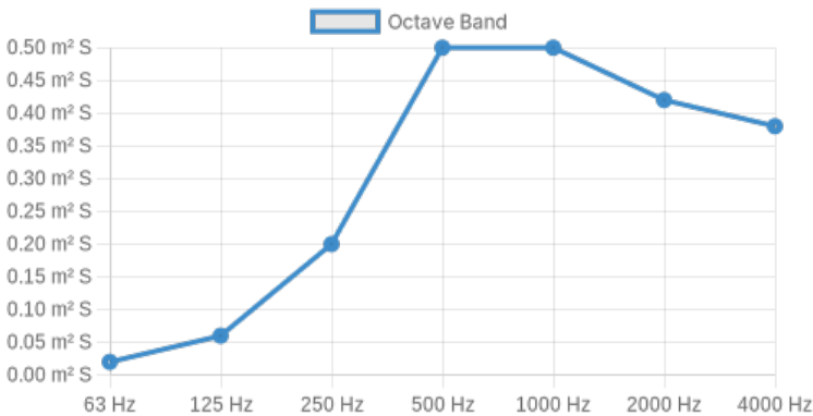
Equivalent sound absorption area per unit
